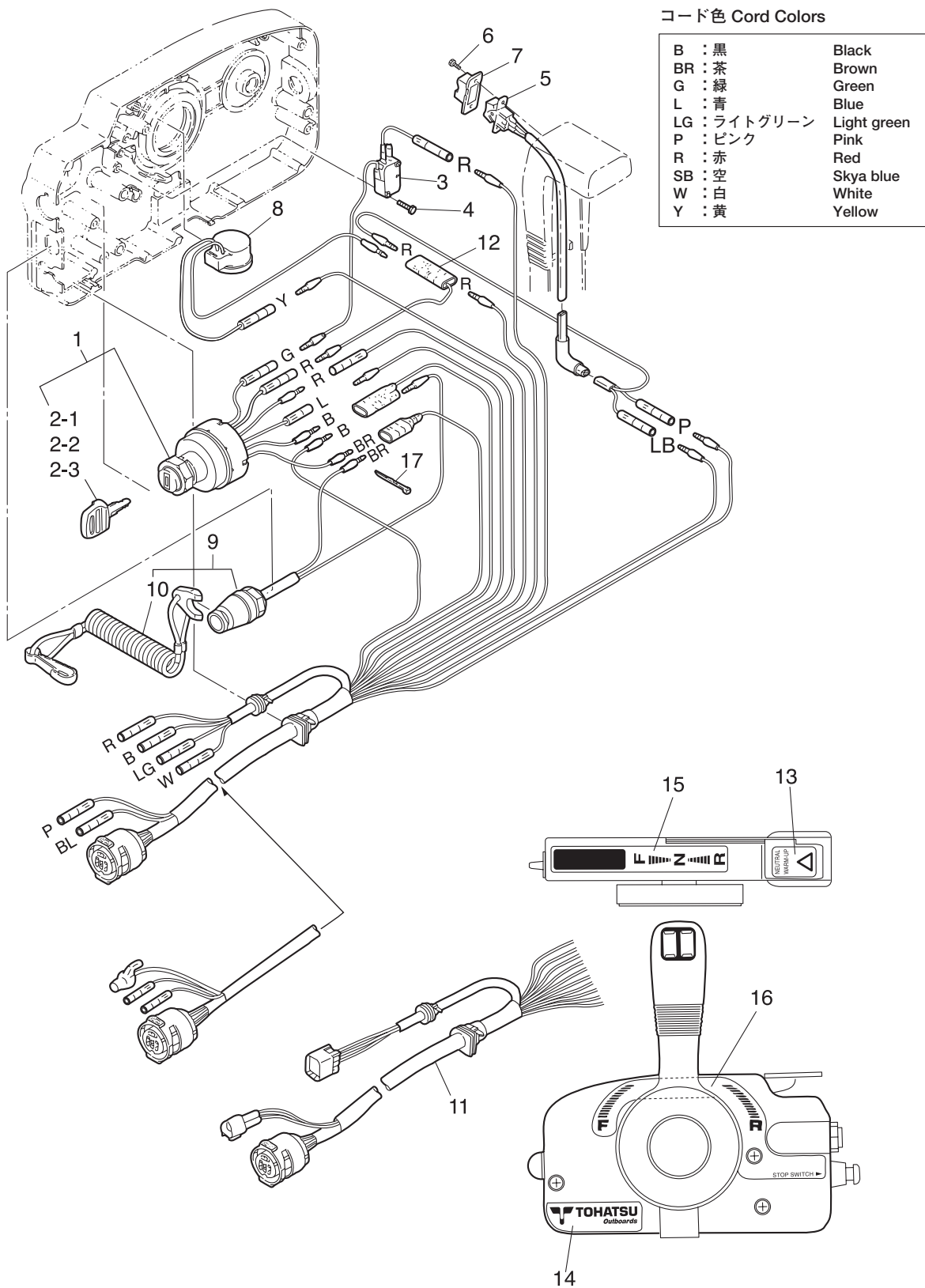
Fig. 28 COMPONENT PARTS OF REMOTE CONTROL BOX (ELECTRICAL PARTS)
